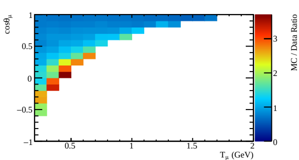
NUWRO v12 / Data Ratio
