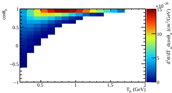
MiniBooNE CCQElike XSec 2DTcos antinu data ( \sigma=2.99\text{E-}37 )
