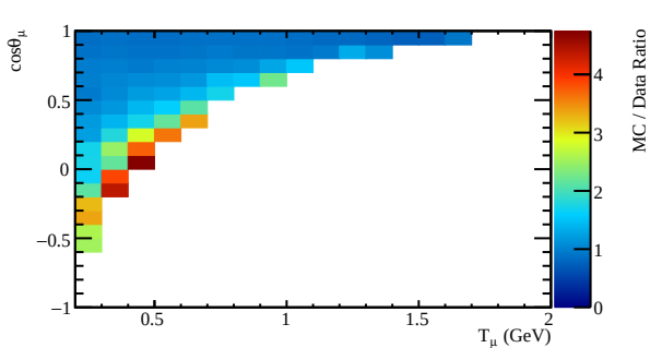
NEUT 5.3.6 / Data Ratio
